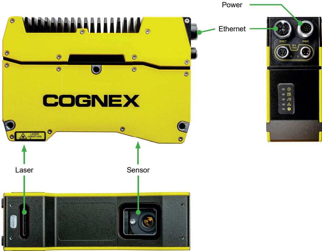
In-Sight L38
