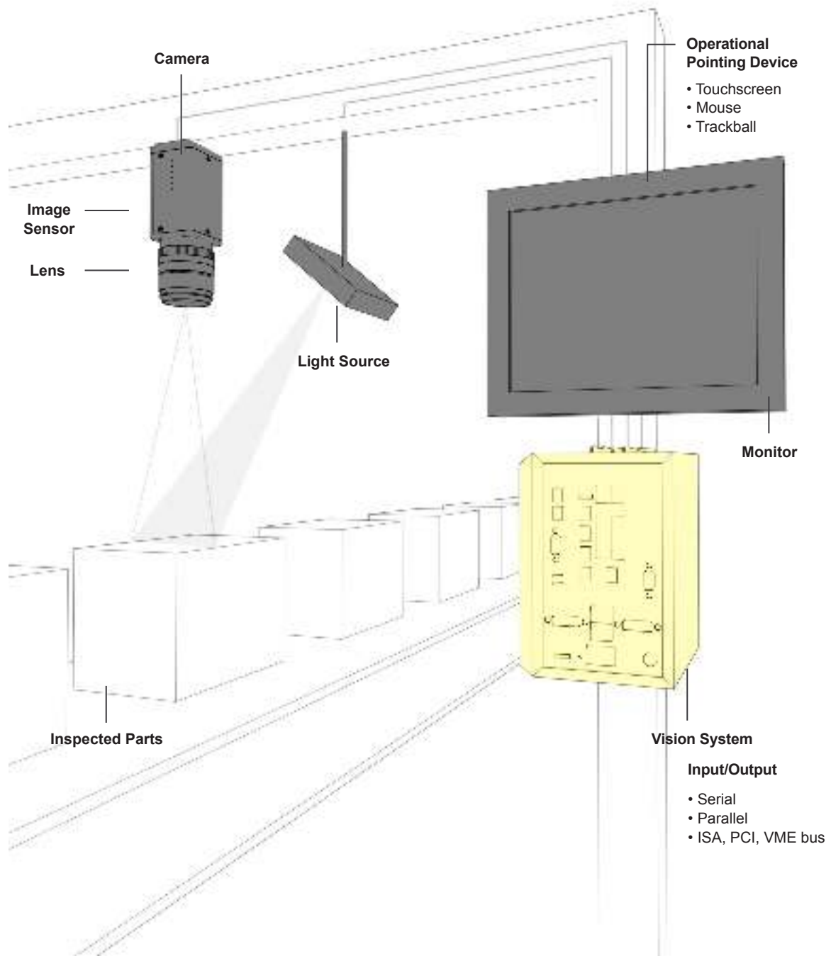
Figure 9. Main components of a machine vision system.
