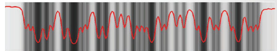
Figure 6. 1-D signal extracted from 1.2 PPM barcode using Hotbars, showing no loss of features
