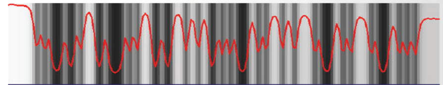
Figure 4b. 1-D signal extracted from 1.5 PPM barcode using bilinear interpolation
