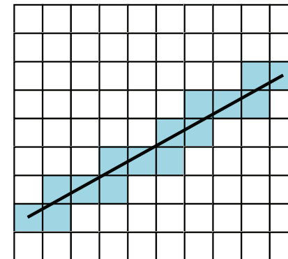
Figure 3. Example of Bresenham line following
